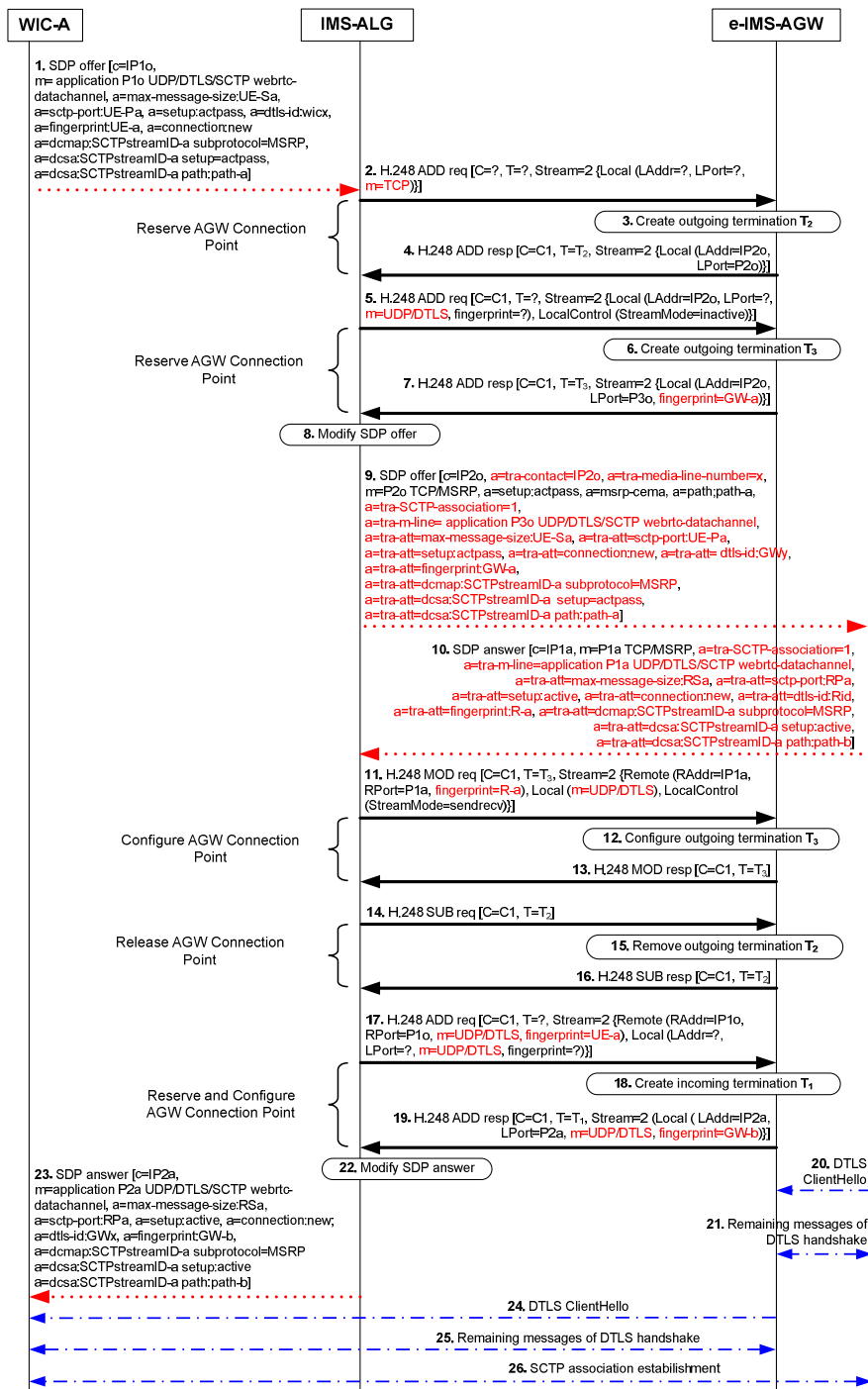
Figure 6.2.22.3.2.1: WIC originated procedure for WebRTC data channel establishment with media plane optimization excluding DTLS layer
