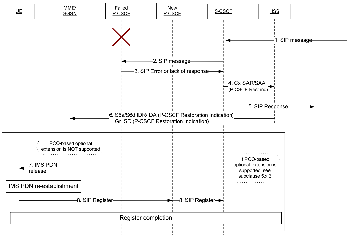
Figure 5.4.2.1-1: HSS-based P-CSCF restoration
