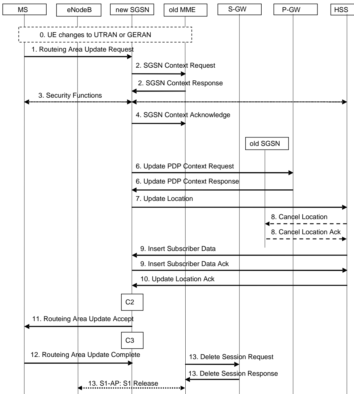
Figure D.3.5-1: Routeing Area Update procedure
