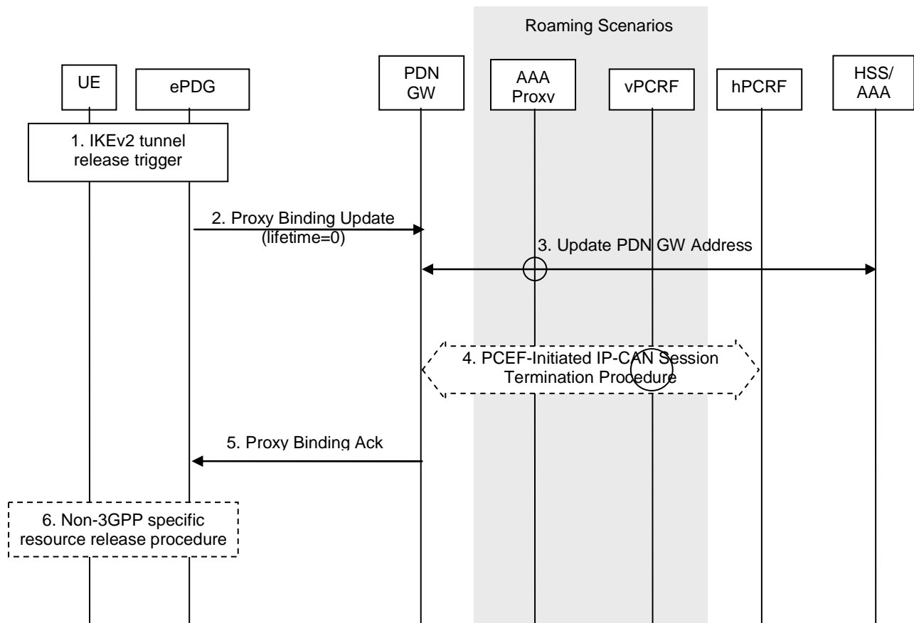
Figure 7.4.1-1: UE/ePDG-initiated detach procedure with PMIPv6
