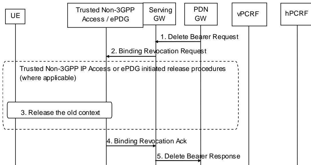
Figure 6.12.4-1 PDN GW initiated Resource Allocation Deactivation for Chained GTP-based S8-S2a/S2b Roaming
