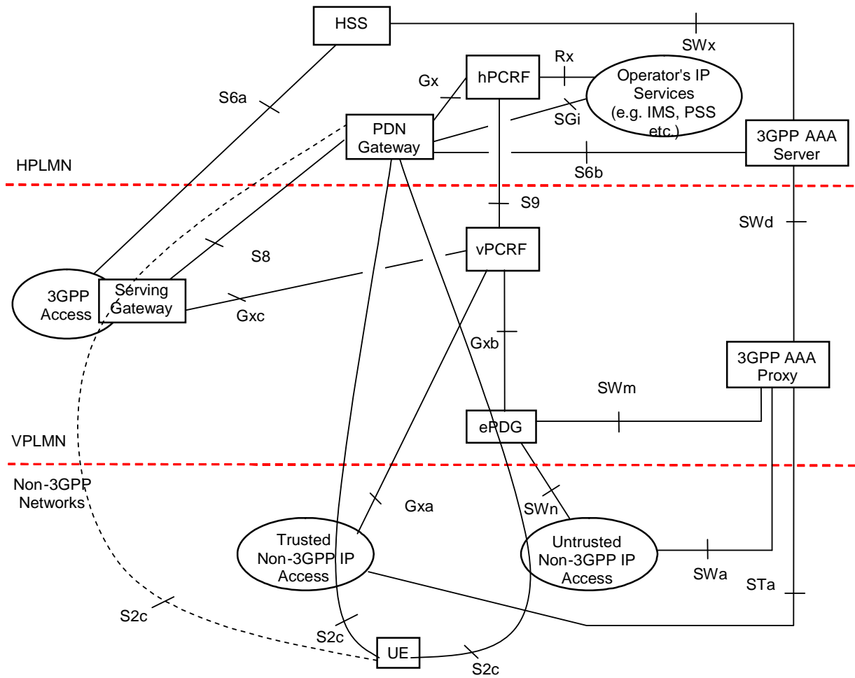
Figure 4.2.3-4: Roaming Architecture for EPS using S8 – S2c - Home Routed
