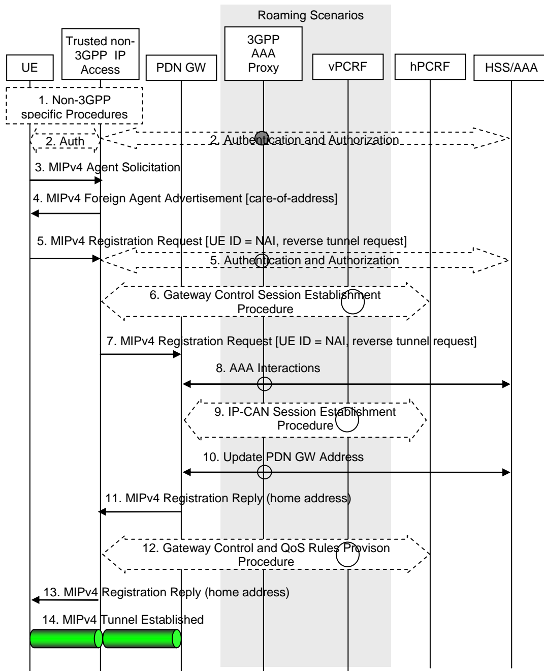
Figure 6.2.3-1: Initial attachment when MIPv4 FCoA mode MM mechanism is used over S2a
