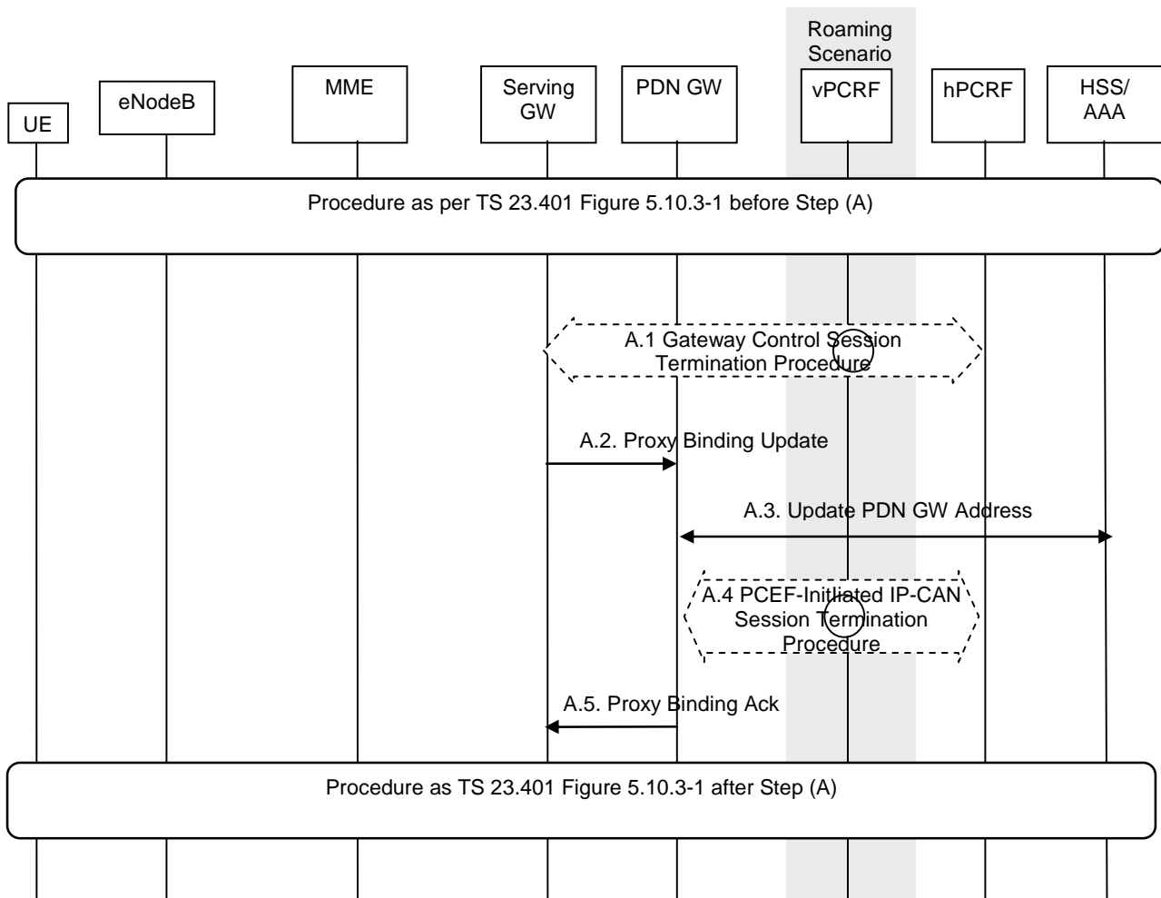
Figure 5.6.1-1: UE requested PDN disconnection Procedure for PMIP-based S5/S8
