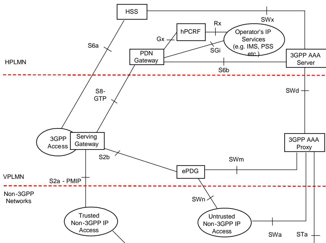
Figure 4.2.3-3: Roaming Architecture for EPS using GTP-based S8, S2a, S2b (Chained GTP-based S8 + S2a-S2b) - Home Routed
