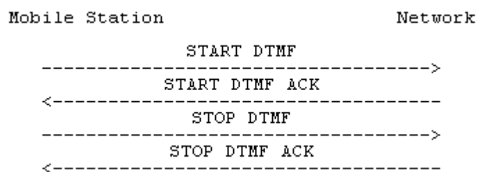
Figure 5.8/3GPP TS 24.008 Single DTMF transmission
