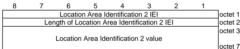
Figure 10.5.5.30/3GPP TS 24.008: Location Area Identification 2 information element
