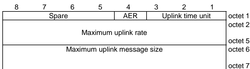
Figure 10.5.136A/3GPP TS 24.008: APN rate control parameters
