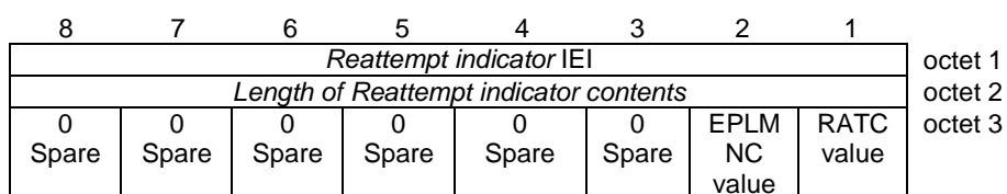
Figure 10.5.6.5A: Re-attempt indicator information element
