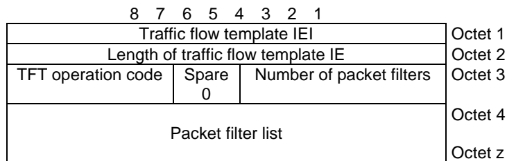
Figure 10.5.144/3GPP TS 24.008: Traffic flow template information element
