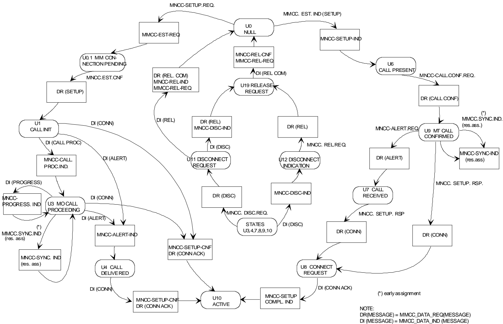
Figure 5.1a/3GPP TS 24.008: Overview call control protocol/MS side
