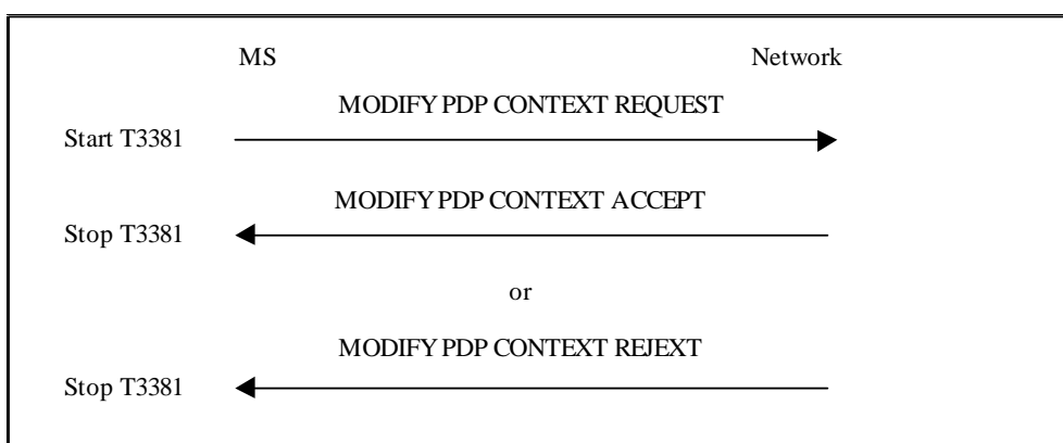
Figure 6.7/3GPP TS 24.008: MS initiated PDP context modification procedure
