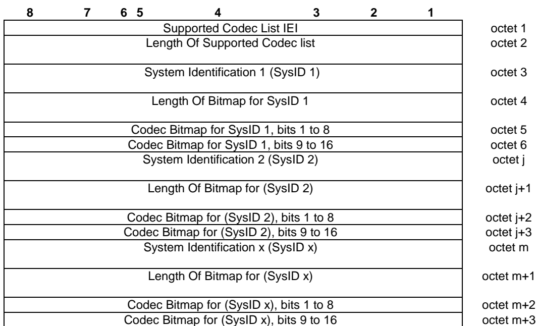
Figure 10.5.118c/3GPP TS 24.008 Supported codec list information element
