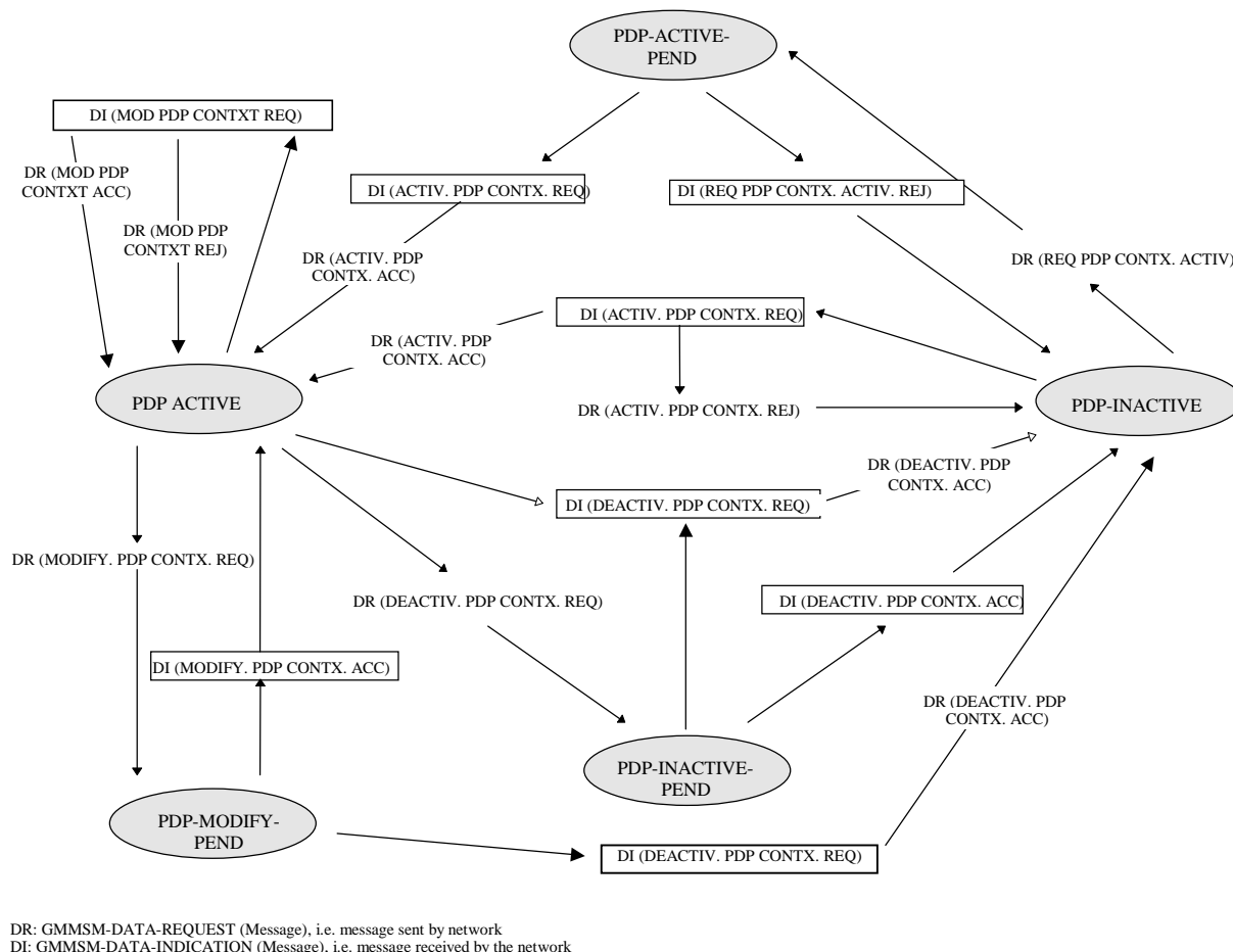
Figure 6.2/3GPP TS 24.008: Session management states on the network side (overview)
