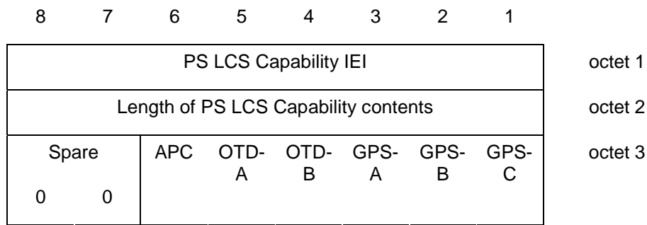
Figure 10.5.135b/3GPP TS 24.008: PS LCS Capability information element
