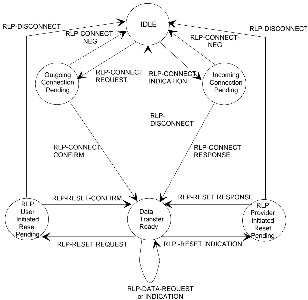
Figure 8: State transition diagram for sequence of RLP connection-mode service primitives
