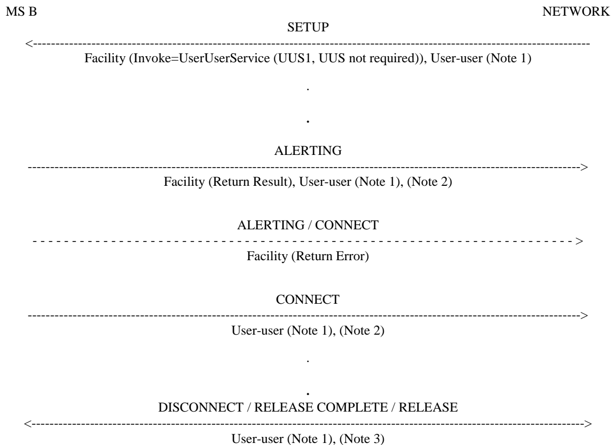
Figure 13: Request for explicit activation of UUS1, UUS not required
