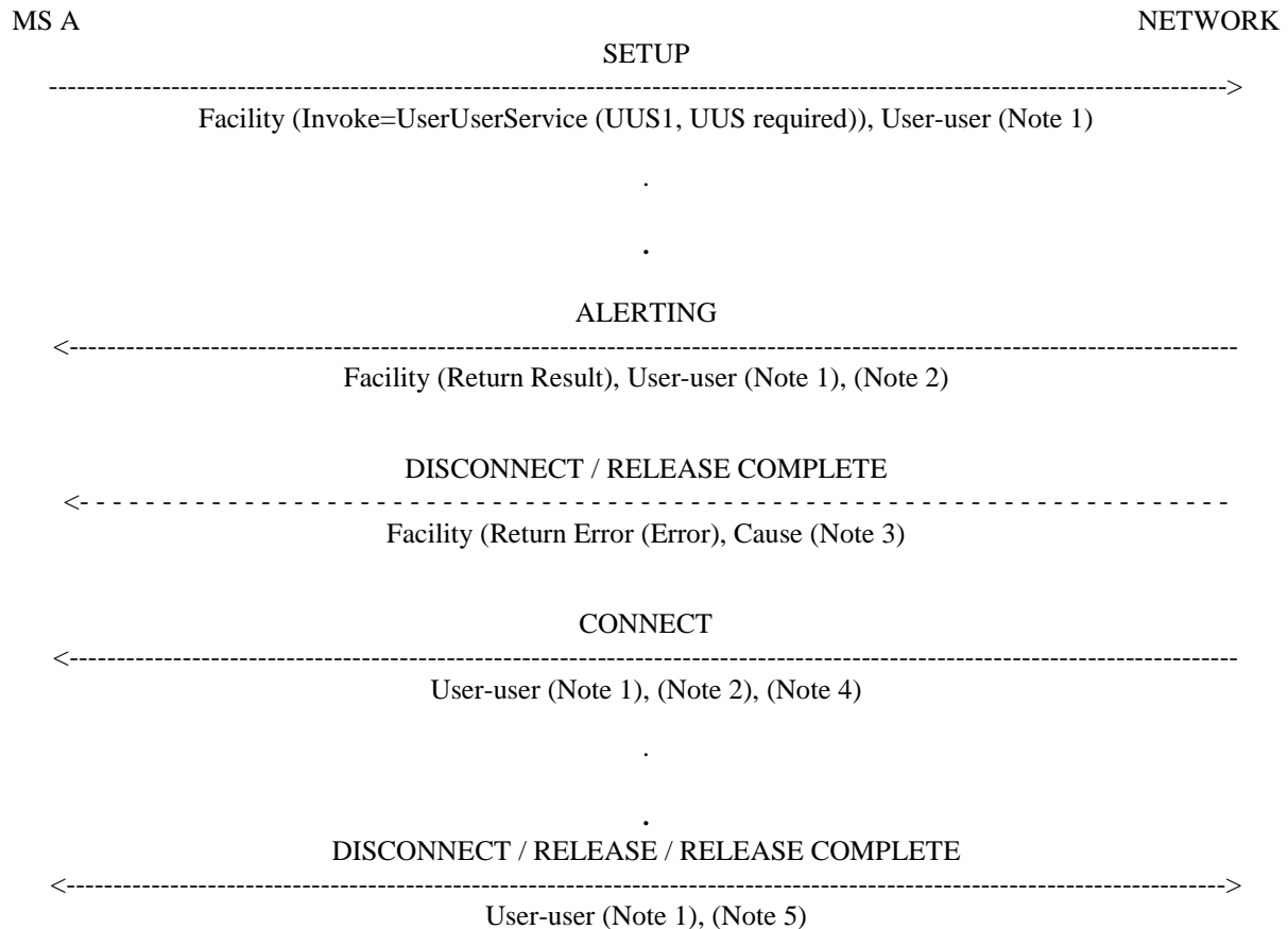
Figure 2: Request for explicit activation of UUS1, UUS required
