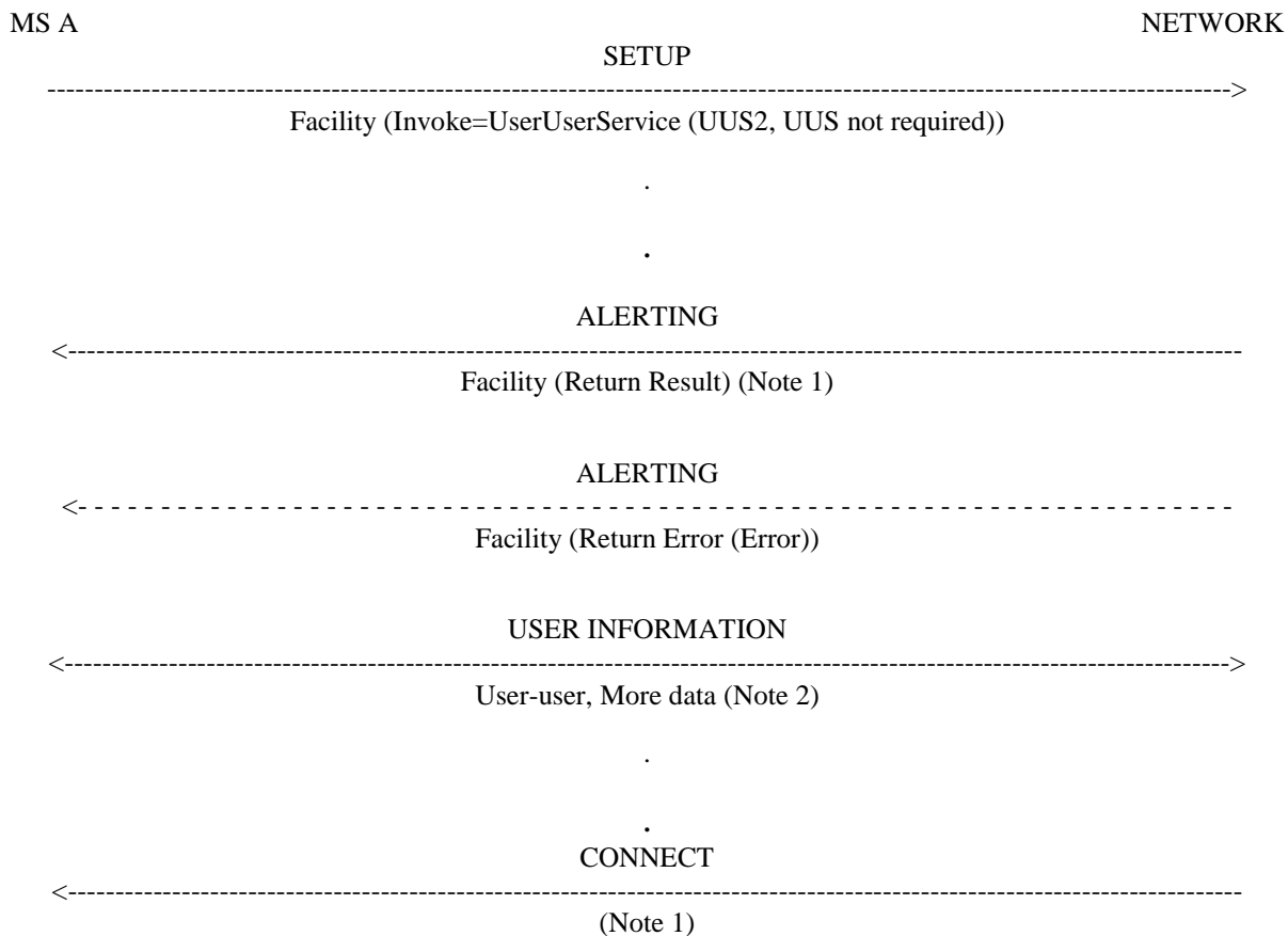
Figure 5: Request for explicit activation of UUS2, UUS not required
