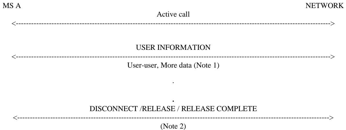
Figure 9: Sending USER INFORMATION messages when UUS3 has been activated
