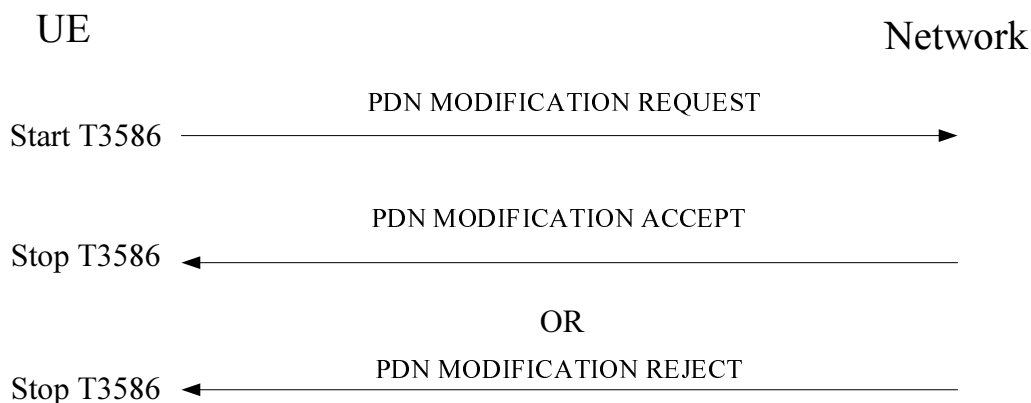
Figure 5.7.2.1: UE-initiated PDN connectivity modification procedure
