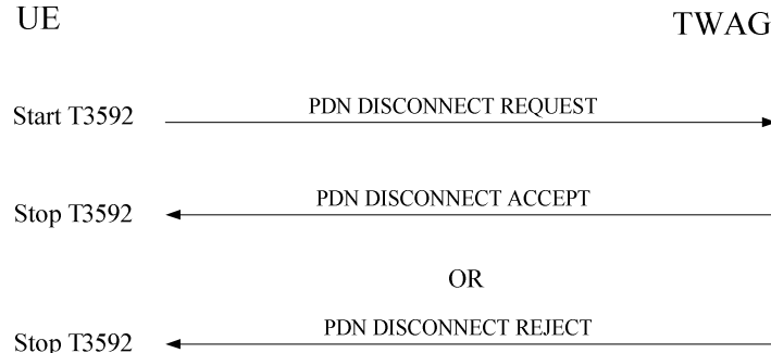
Figure 5.4.2.1: UE requested PDN disconnection procedure
