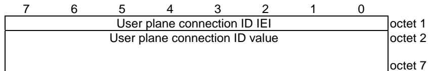
Figure 8.10.1: User plane connection ID information element
