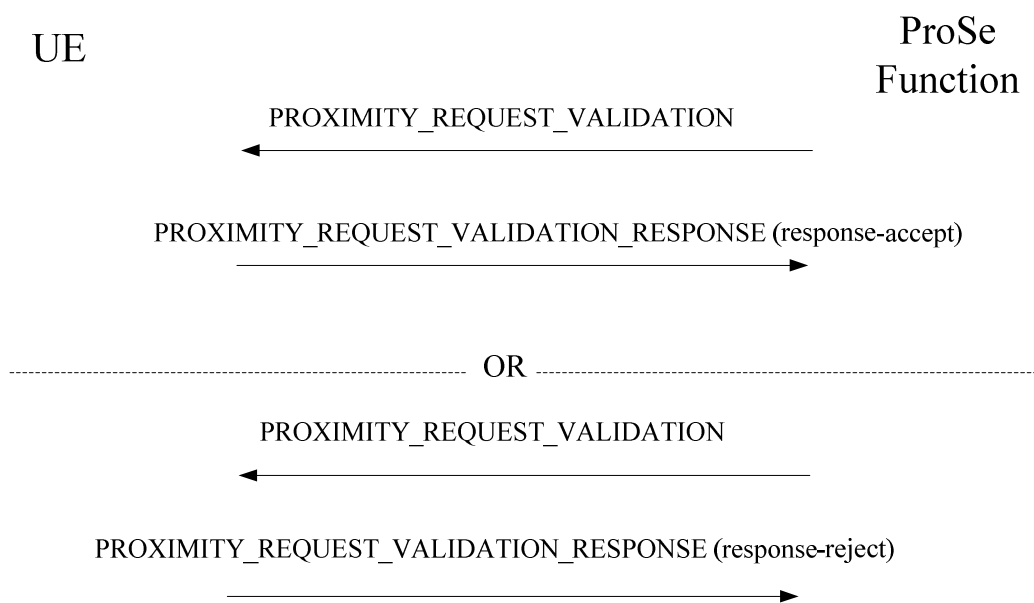
Figure 7.2.8.2.1: Proximity request validation procedure
