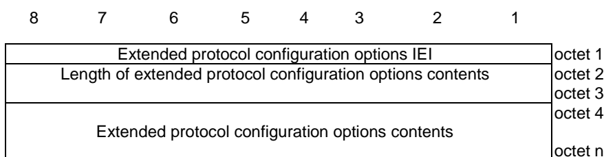
Figure 9.9.4.26.1: Extended protocol configuration options information element
