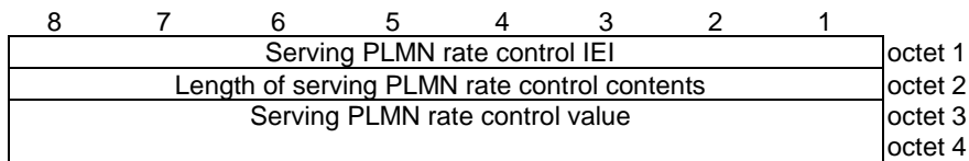
Figure 9.9.4.28.1: Serving PLMN rate control information element
