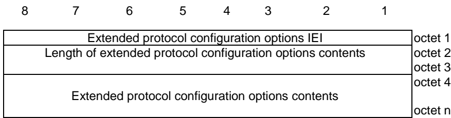
Figure 9.9.4.26.1: Extended protocol configuration options information element
