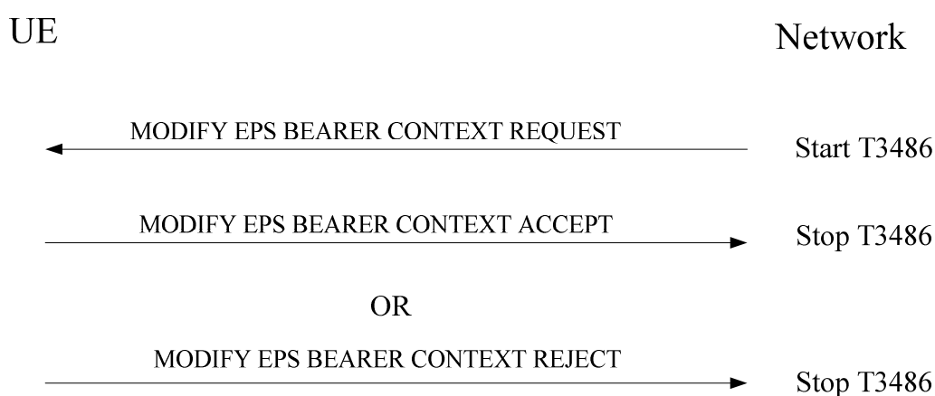
Figure 6.4.3.2.1: EPS bearer context modification procedure
