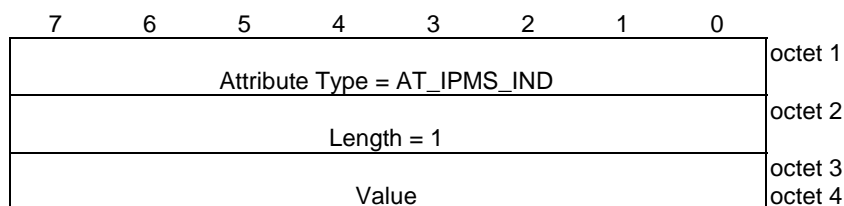
Figure 8.2.1.1: AT_IPMS_IND attribute
