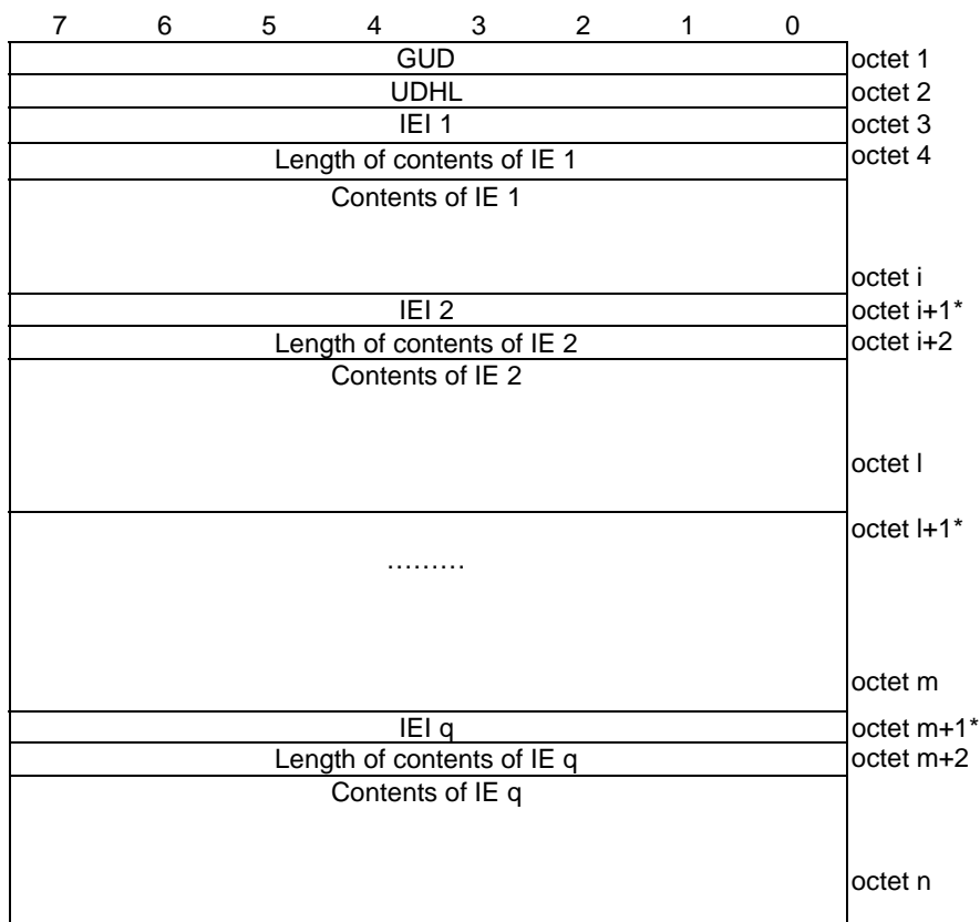
Figure H.2.1-1 – Structure of IEEE Std 802.11u-2011 Generic Container
