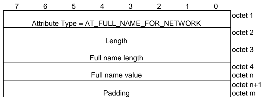
Figure 8.2.5.1-1: AT_FULL_NAME_FOR_NETWORK attribute
