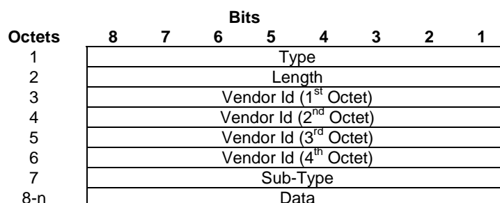
Figure A.2-1: 3GPP Vendor-Specific Mobility Option
