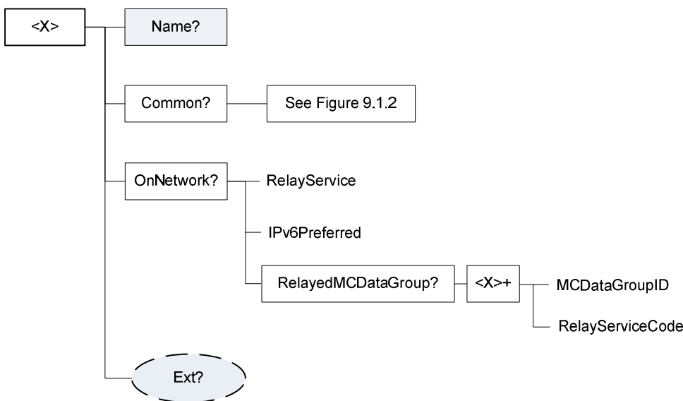
Figure 9.1.1: The MCDATA UE configuration MO (1 of 2)
