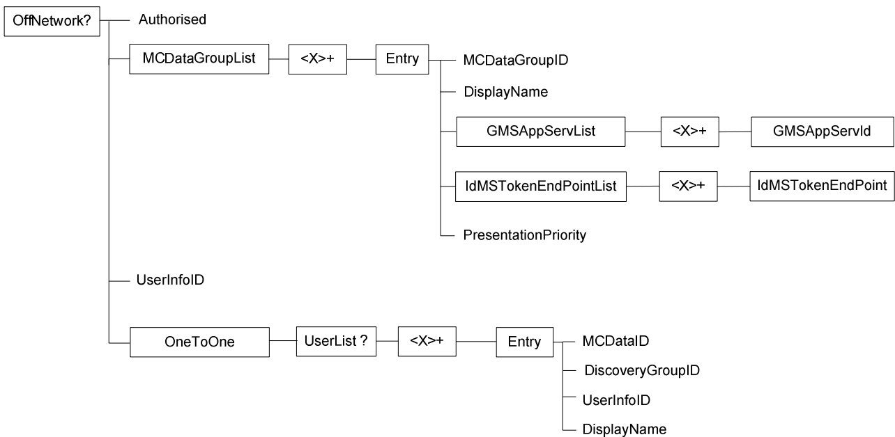
Figure 10.1.3: The MCDATA user profile MO (3 of 3)
