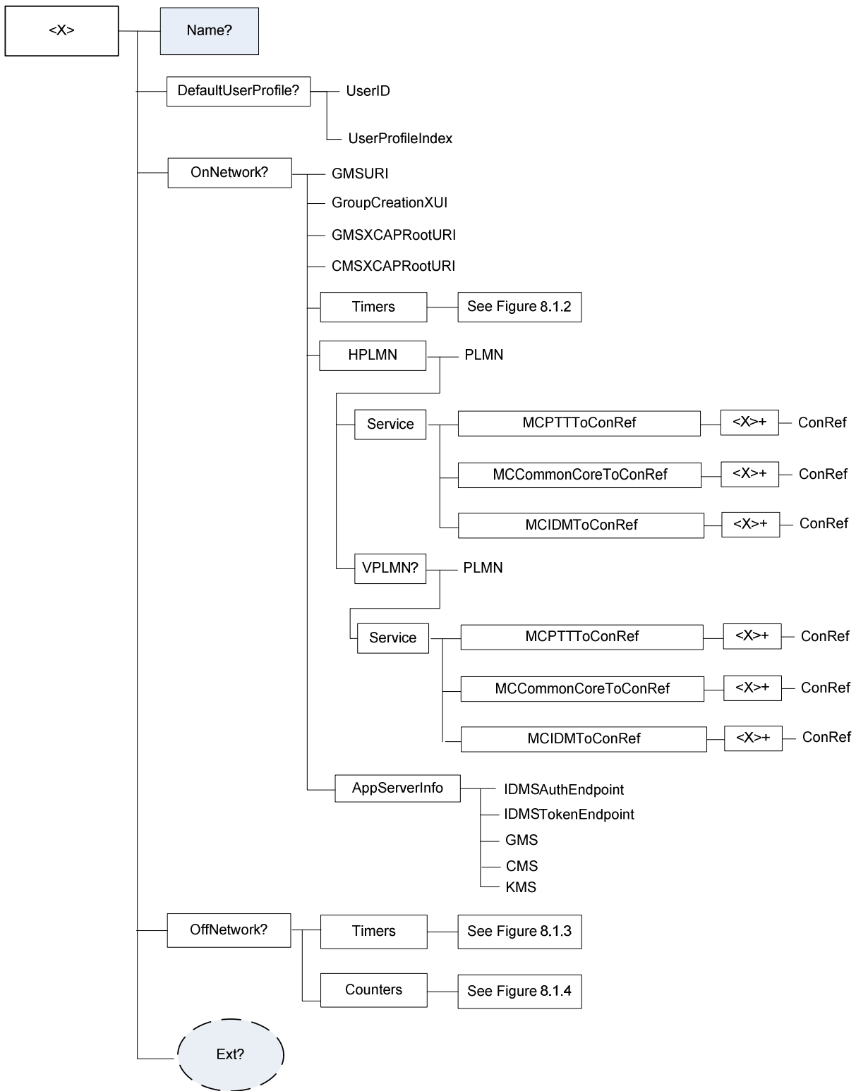
Figure 8.1.1: The MCS UE initial configuration MO (1 of 4)
