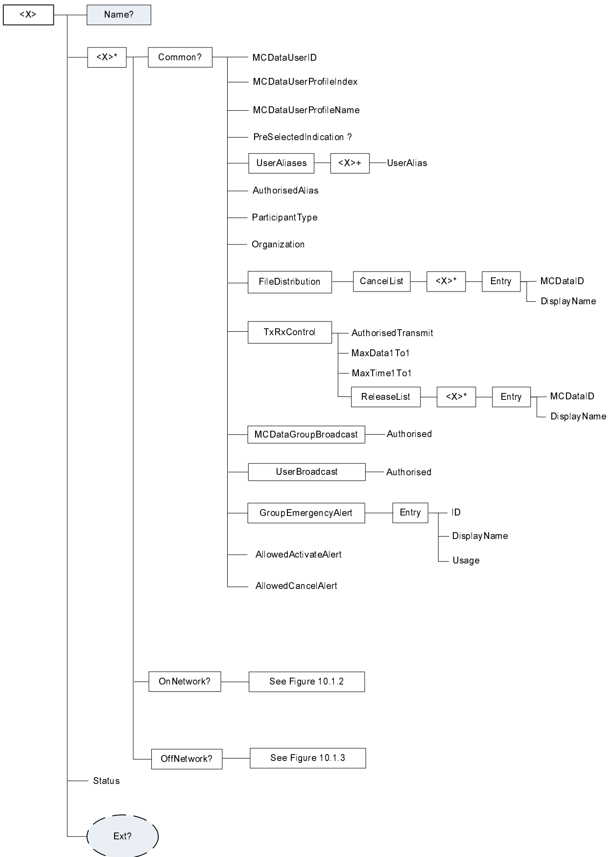
Figure 10.1.1: The MCDATA user profile MO (1 of 3)
