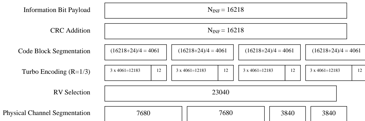
Figure A.19B. S-E-DPDCH
