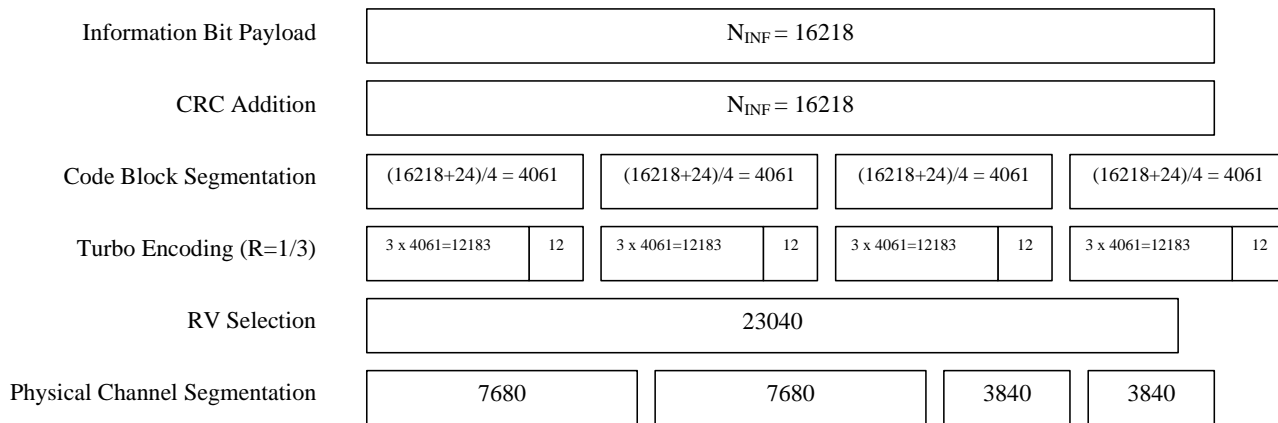
Figure A.19A. E-DPDCH
