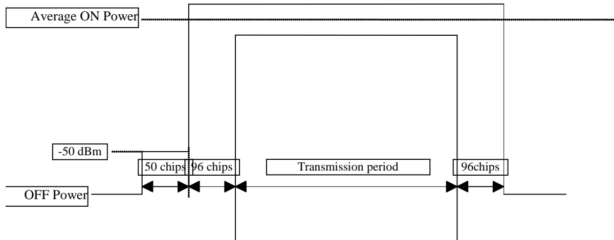
Figure 6.2: Transmit ON/OFF template
