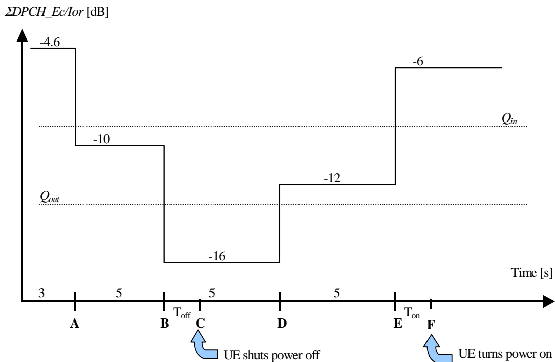
Figure 6.1. Test case for out-of-synch handling in the UE.– continuous transmission
