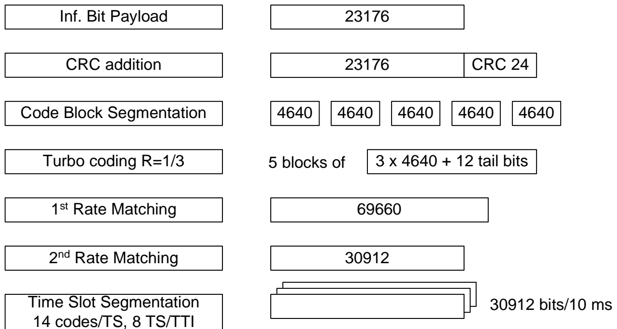
Figure A.10: Coding for HS-PDSCH fixed reference channel with QPSK modulation for the VA120 Channel - Category 8
