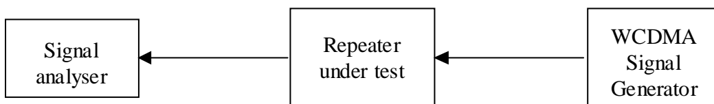
Figure A.7: Measuring system set-up for modulation accuracy: peak code domain error error and relative code domain error.
