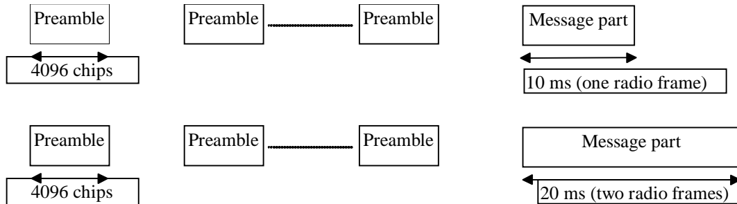
Figure 4: Structure of the random-access transmission
