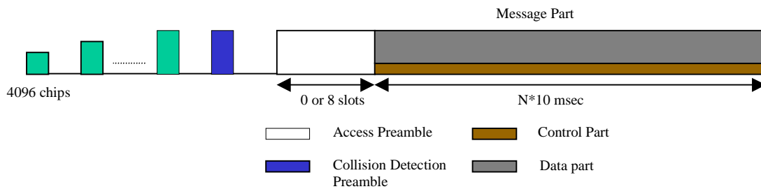
Figure 6: Structure of the CPCH access transmission
