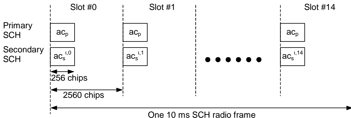
Figure 20: Structure of Synchronisation Channel (SCH)
