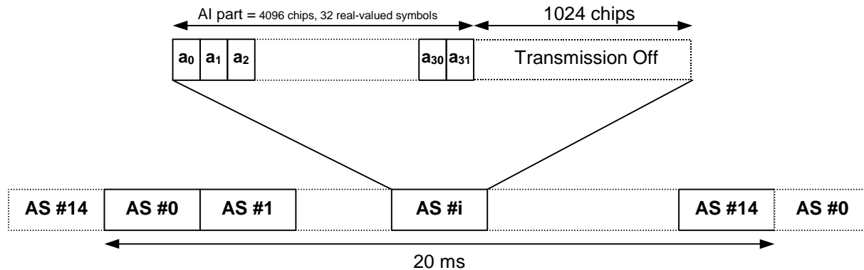
Figure 23: Structure of Acquisition Indicator Channel (AICH)
