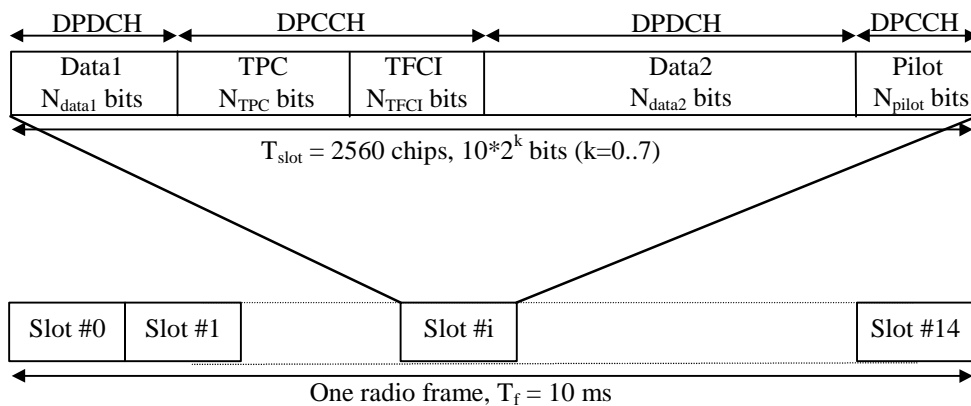
Figure 11: Frame structure for downlink DPCH
