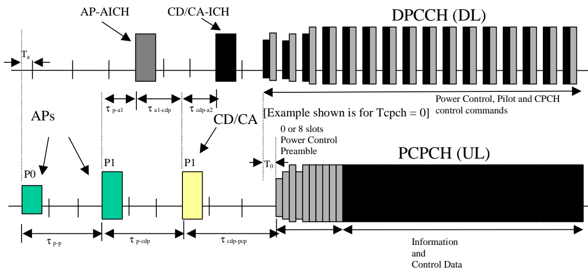
Figure 36: Timing of PCPCH and AICH transmission as seen by the UE, with T_{cpch} = 0
