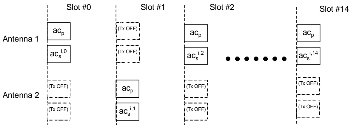
Figure 21: Structure of SCH transmitted by TSTD scheme
