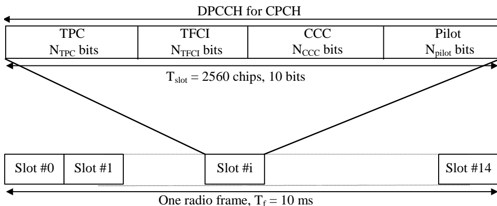
Figure 14: Frame structure for downlink DPCCH for CPCH
