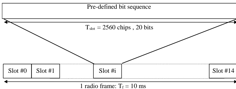
Figure 15: Frame structure for Common Pilot Channel
