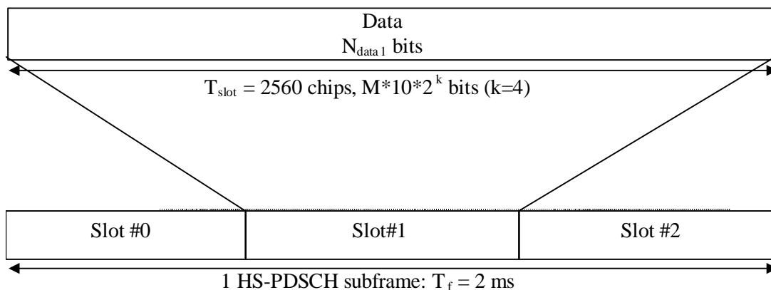
Figure 30: Subframe structure for the HS-PDSCH
