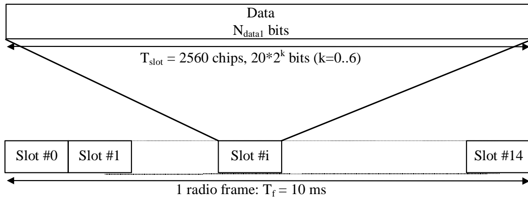
Figure 22: Frame structure for the PDSCH
