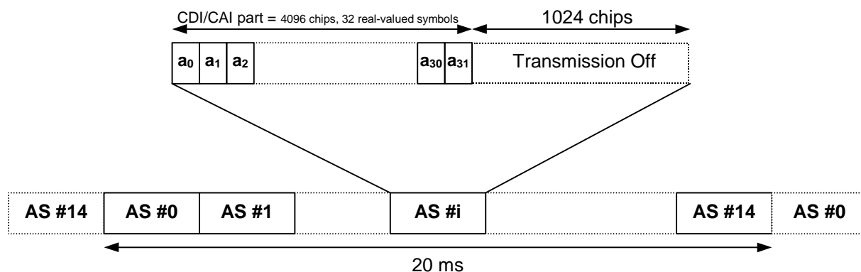
Figure 25: Structure of CD/CA Indicator Channel (CD/CA-ICH)
