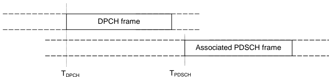
Figure 37: Timing relation between DPCH frame and associated PDSCH frame
