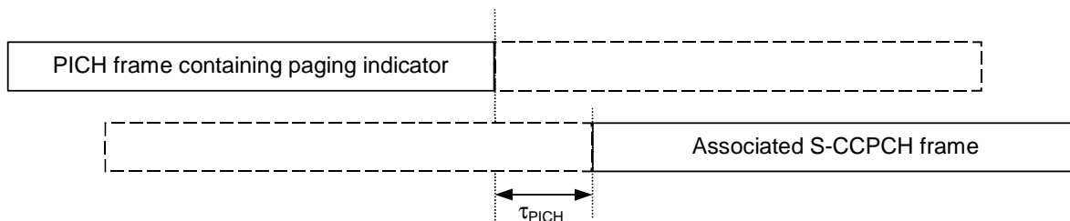
Figure 34: Timing relation between PICH frame and associated S-CCPCH frame
