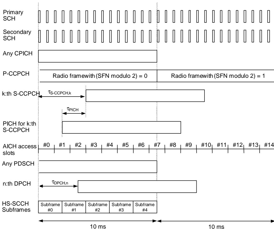
Figure 33: Radio frame timing and access slot timing of downlink physical channels
