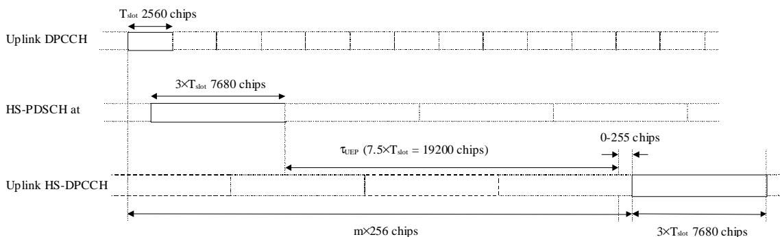
Figure 38: Timing structure at UE for HS-DPCCH control signalling
