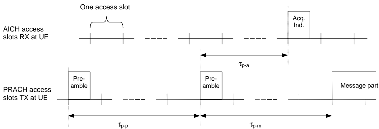
Figure 35: Timing relation between PRACH and AICH as seen at the UE
