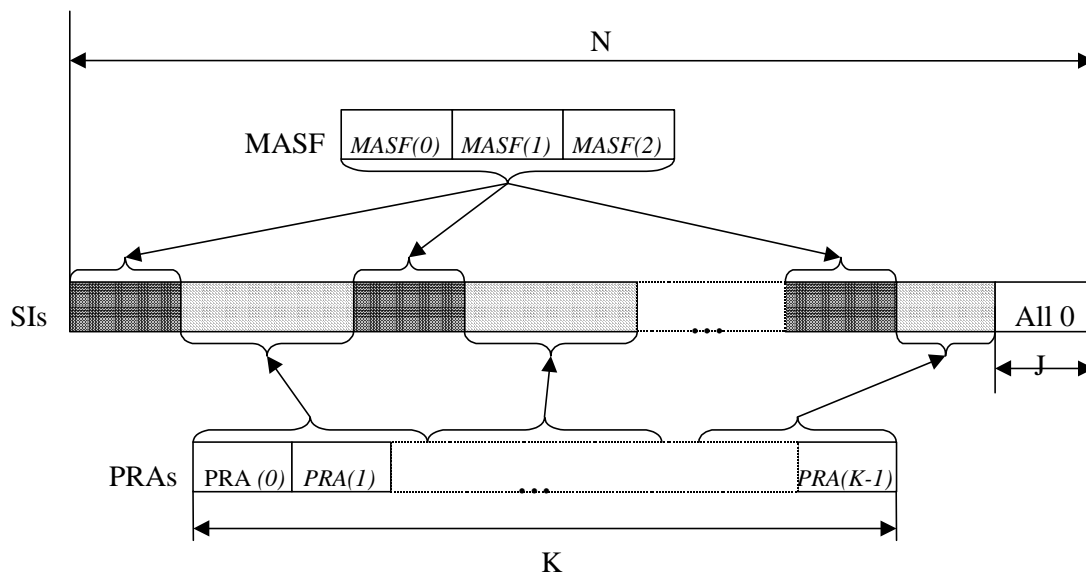
Figure 28: Mapping of MASF and PRAs to SIs in CSICH
