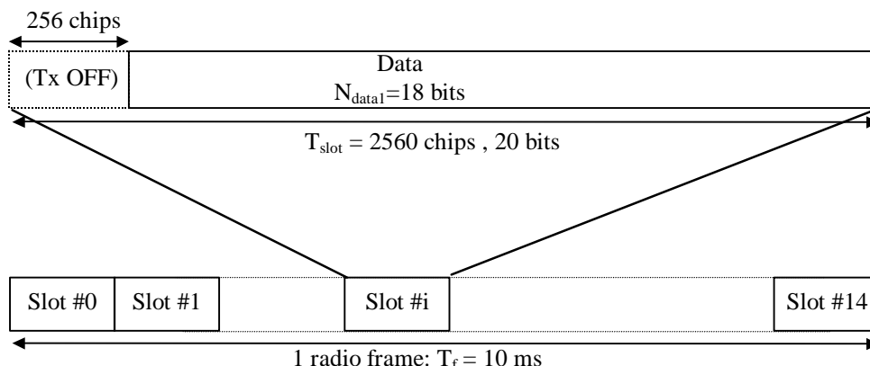
Figure 17: Frame structure for Primary Common Control Physical Channel
