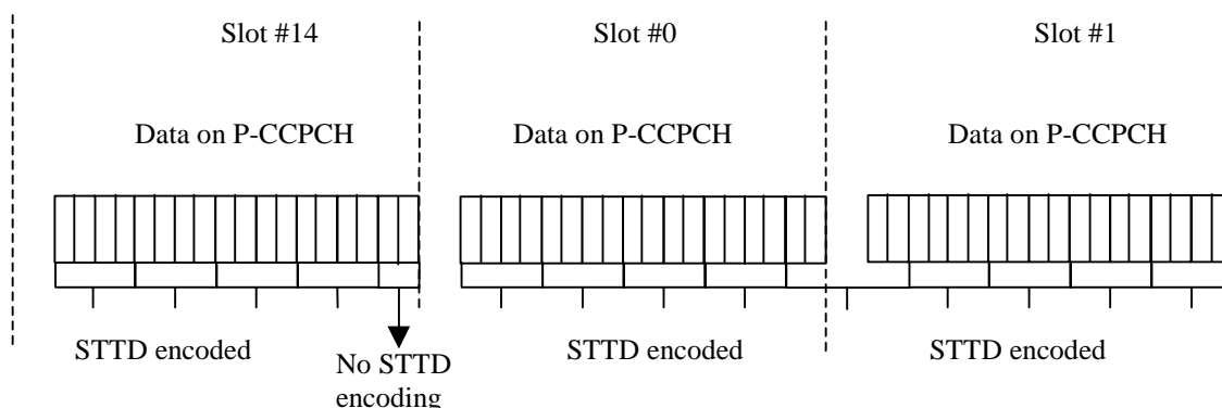
Figure 18: STTD encoding for the data bits of the P-CCPCH
