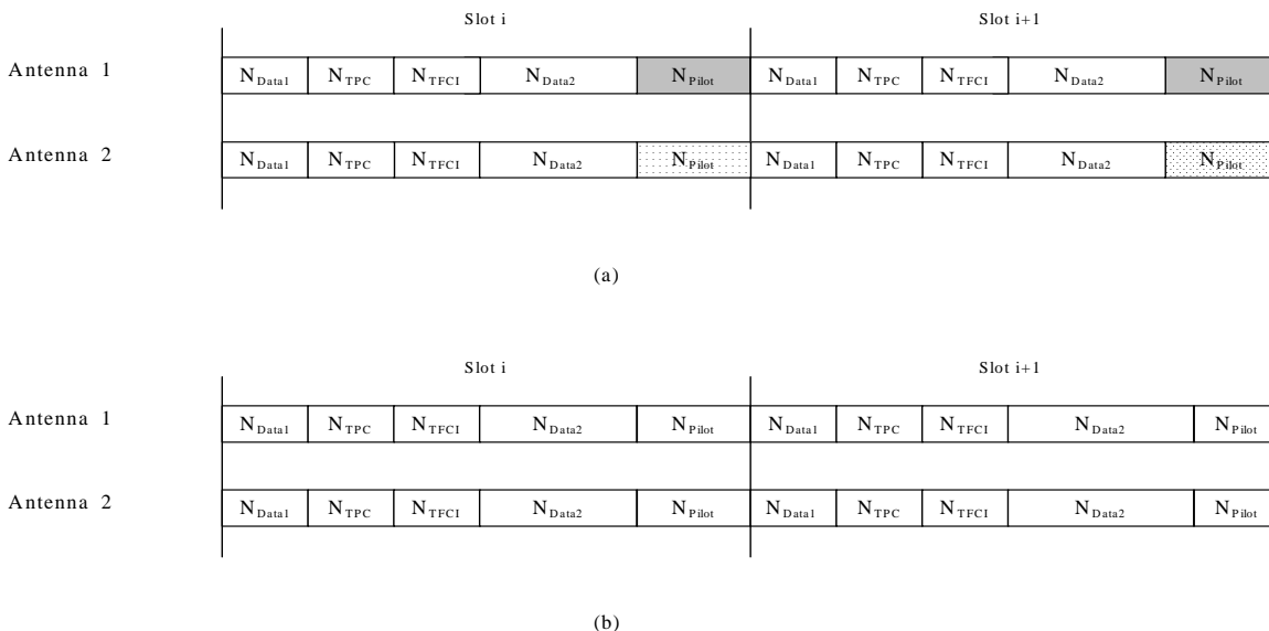
Figure 13: Slot structures for downlink dedicated physical channel diversity transmission. Structure (a) is used in closed loop mode 1. Structure (b) is used in closed loop mode 2. Different shading of the pilots indicate orthogonality of the patterns
