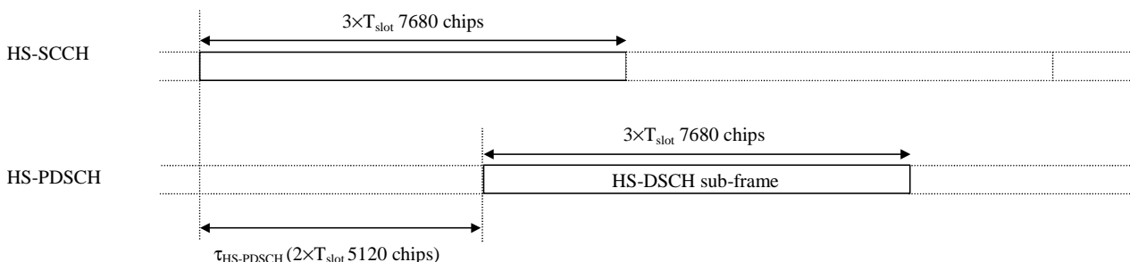
Figure 39: Timing relation between the HS-SCCH and the associated HS-PDSCH.
