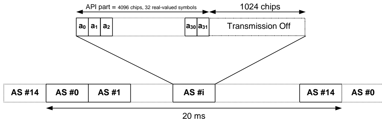
Figure 24: Structure of AP Acquisition Indicator Channel (AP-AICH)
