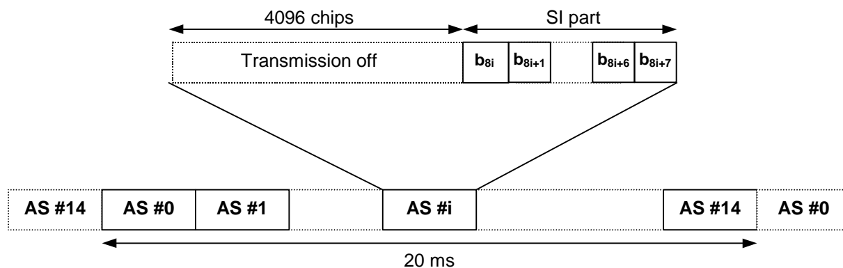
Figure 27: Structure of CPCH Status Indicator Channel (CSICH)
