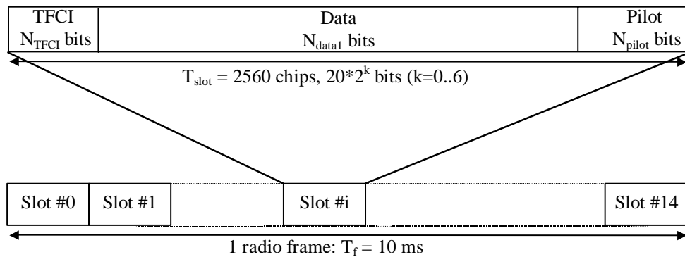
Figure 19: Frame structure for Secondary Common Control Physical Channel
