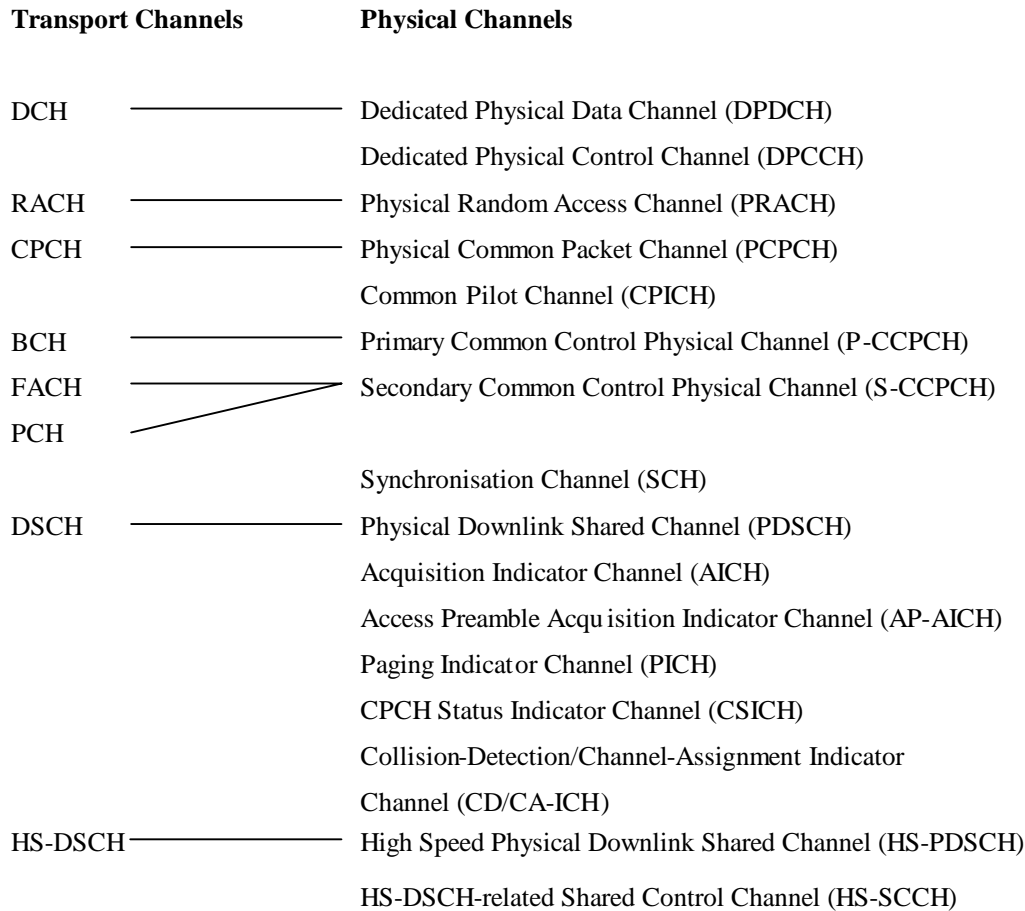
Figure 31: Transport-channel to physical-channel mapping
