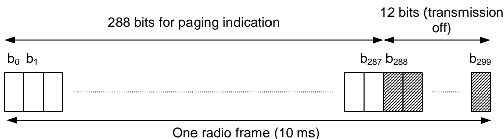
Figure 26: Structure of Paging Indicator Channel (PICH)
