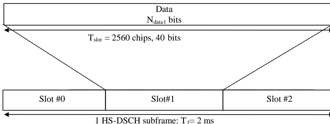
Figure 29: Subframe structure for the HS-SCCH
