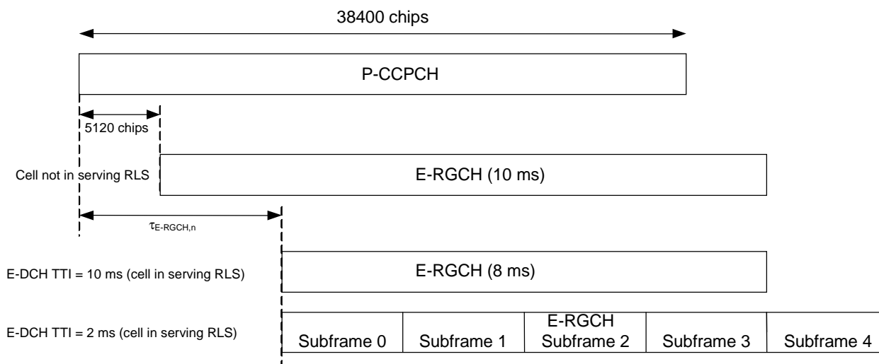
Figure 38: E-RGCH timing
