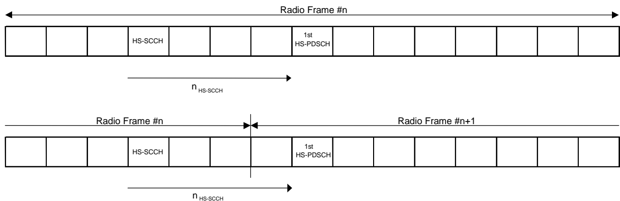
Figure 21A: Timing for HS-SCCH and HS-PDSCH for different radio frame configurations for a given UE
