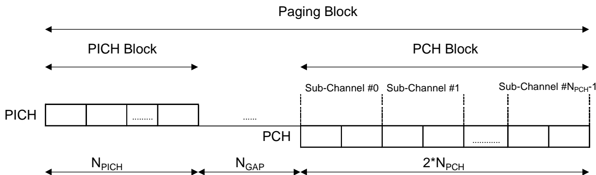
Figure 20: Paging Sub-Channels and Association of PICH and PCH blocks
