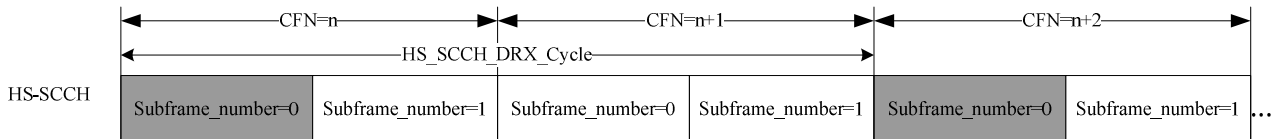
Figure 11B: Example for HS-SCCH reception pattern
