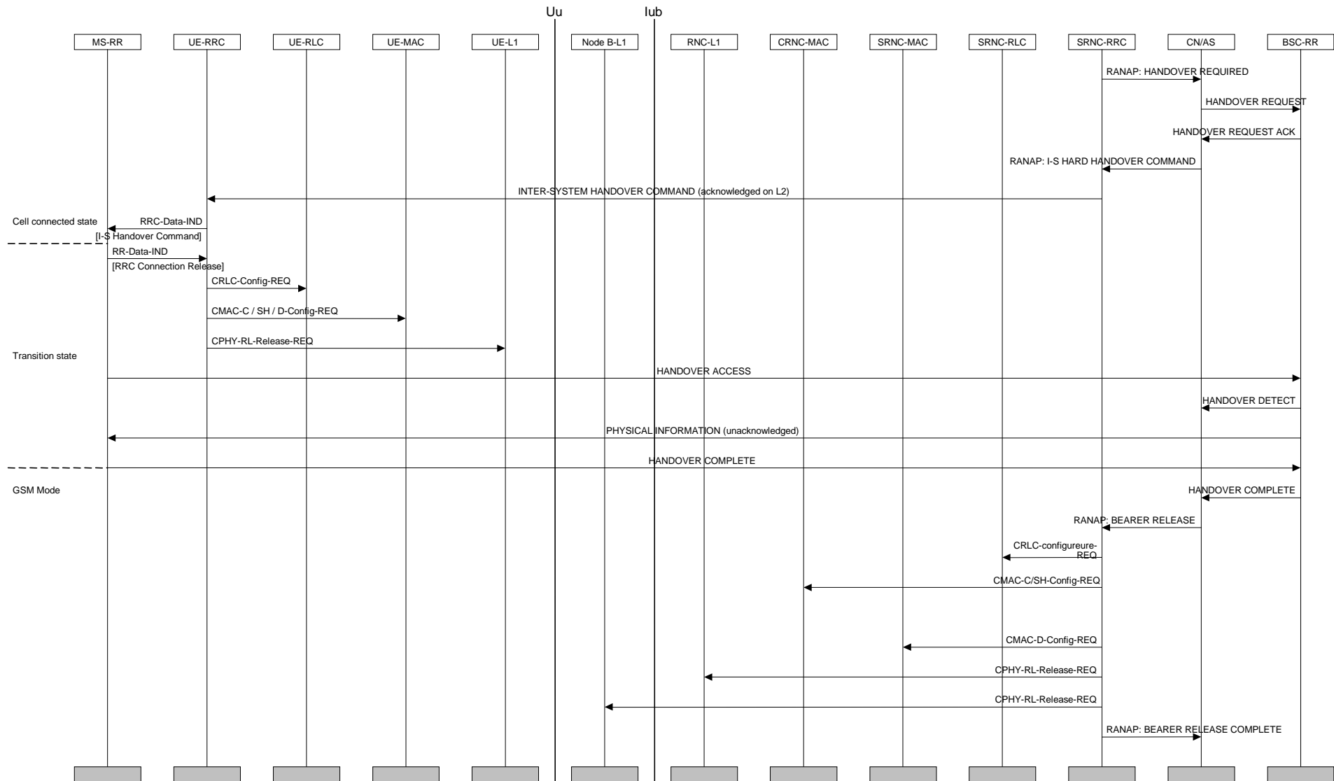
Figure 40: UMTS to GSM inter-system handover
