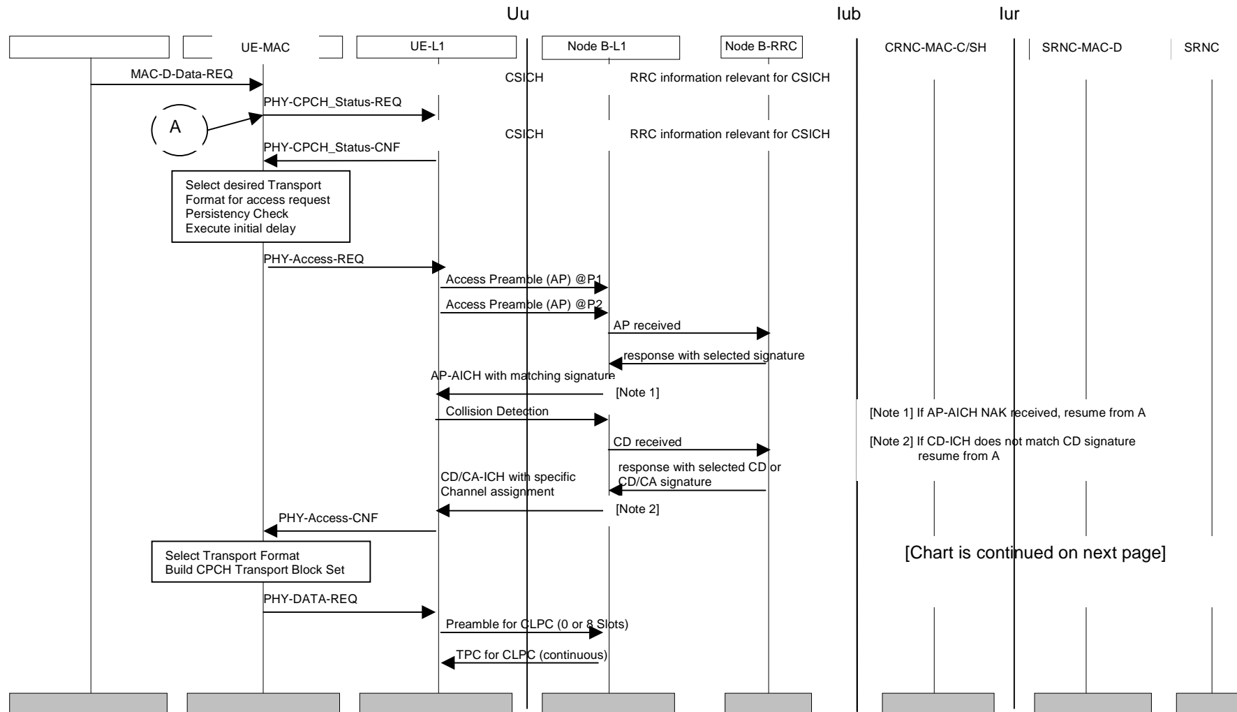
Figure 21: Example of data transmission on CPCH (page 1 of 2)
