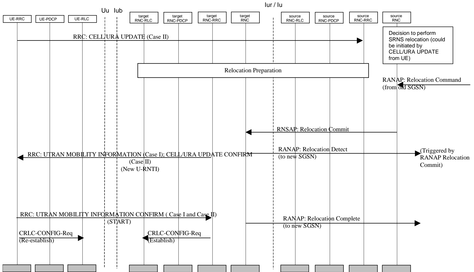
Figure 36: Serving and Combined Cell/URA Update SRNS relocation (seamless radio bearers)
