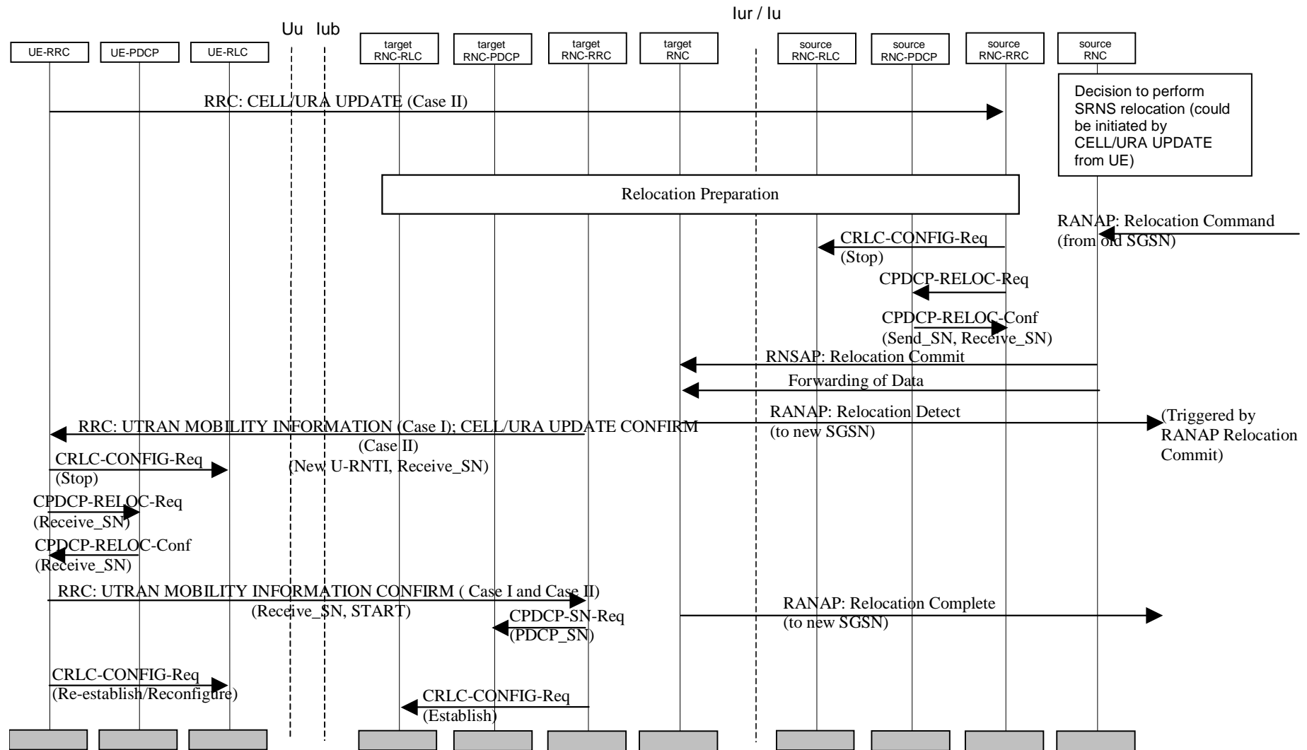
Figure 34: Serving and Combined Cell/URA Update SRNS relocation (lossless radio bearers)
