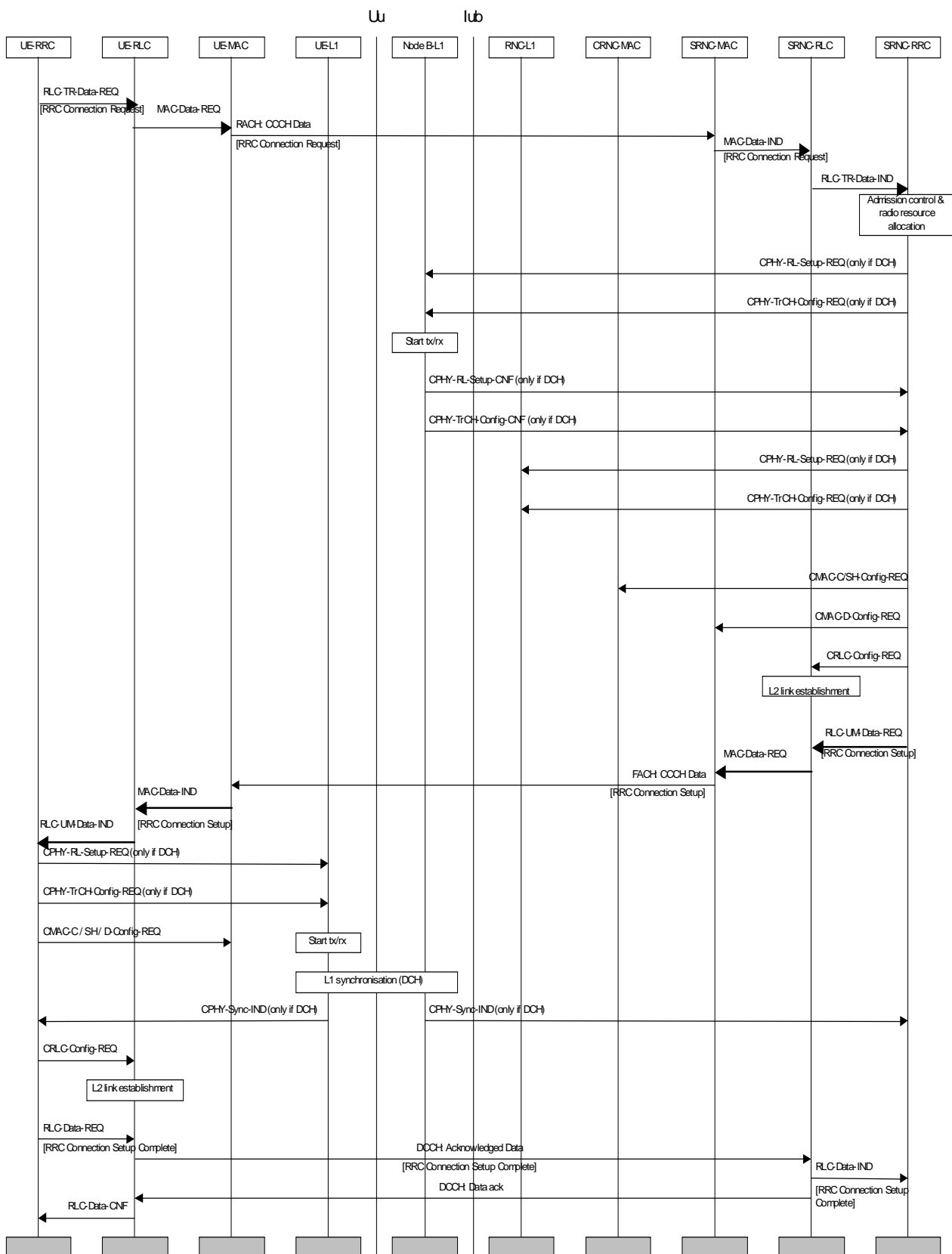
Figure 1: RRC connection establishment (with common channel termination case A)
