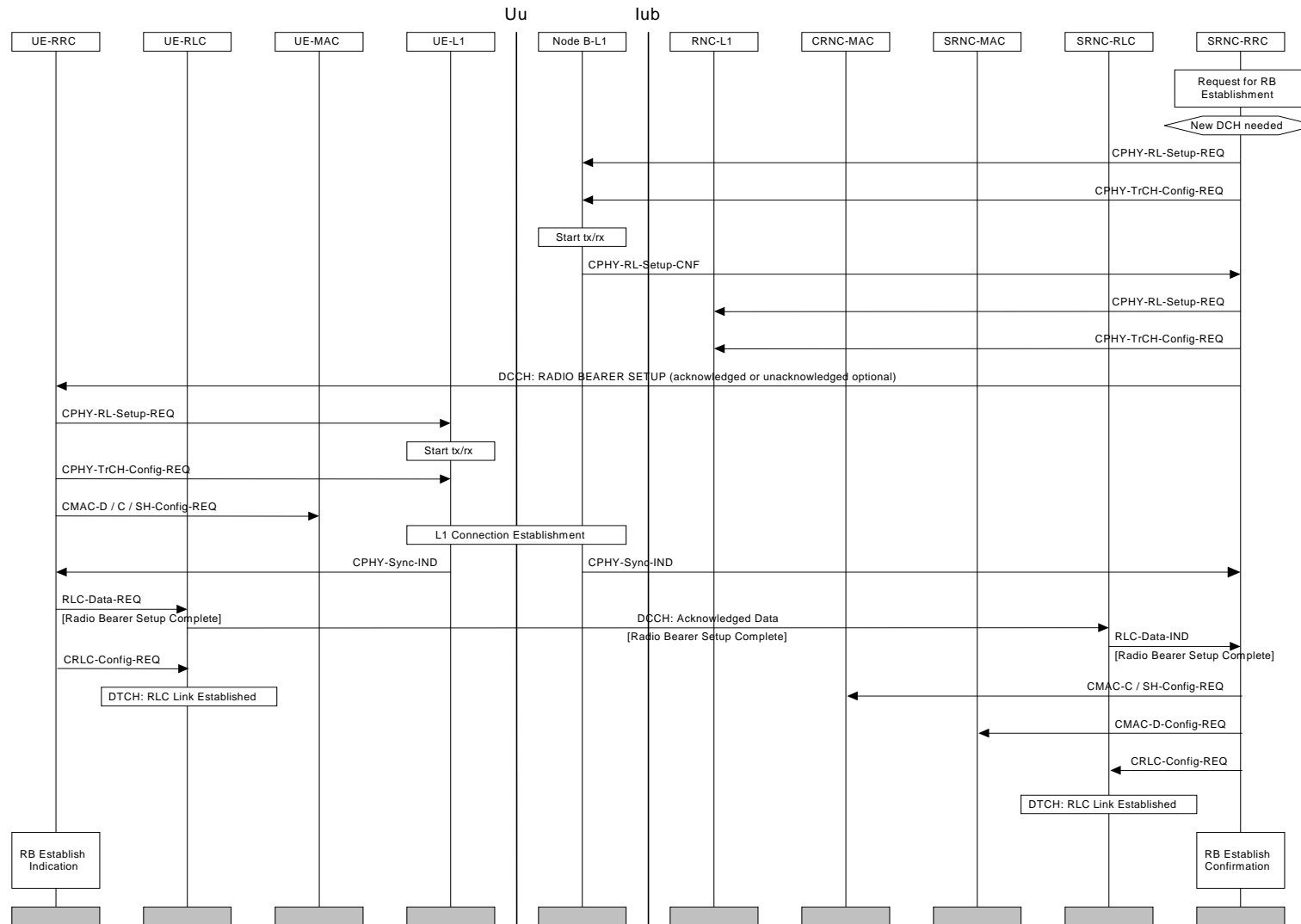
Figure 5: Radio Bearer Establishment with Dedicated Physical Channel Activation
