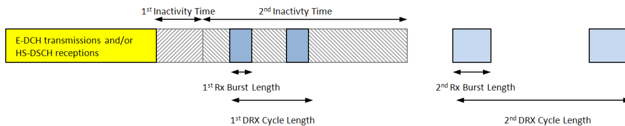
Figure 14.4.2-1: Discontinuous HS-DSCH reception with second DRX cycle in CELL_FACH state
