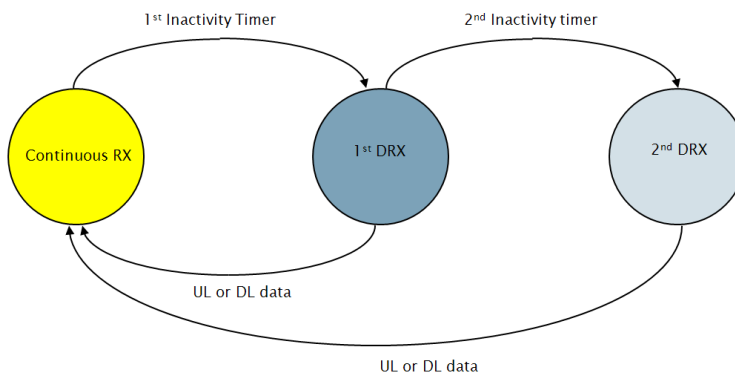
Figure 14.4.2-0a: HS-DSCH DRX in CELL_FACH with 2-level DRX
