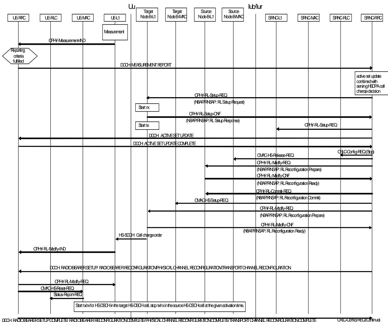
Figure 9.6-1: Inter-Node B serving HS-DSCH cell change with target cell pre-configuration
