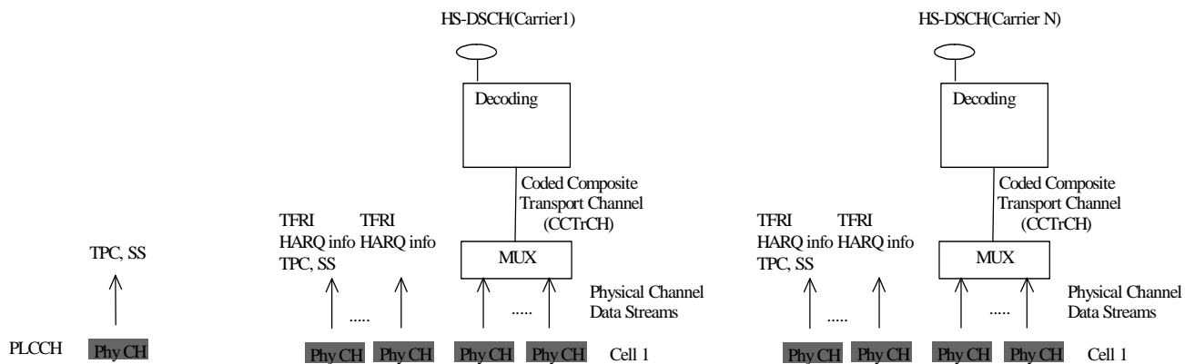
Figure 5.2.2.2-3: Model of the UE's physical layer in CELL_DCH state (1.28Mcps TDD multi-frequency HS-DSCH operation mode only)
