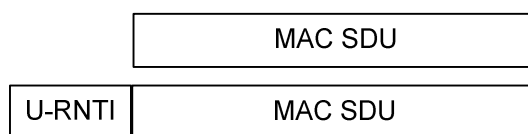
Figure 9.2.1.1c-1: MAC-d/MAC-c PDU format for DTCH and DCCH mapped on HS-DSCH (FDD and 1.28 Mcps TDD only)
