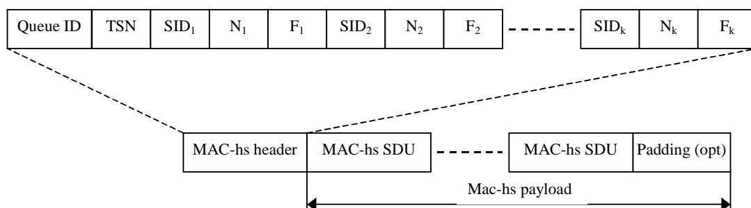
Figure 9.1.4.1: MAC-hs PDU
