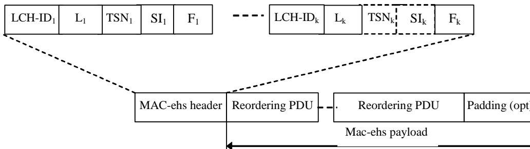
Figure 9.1.4.2: MAC-ehs PDU
