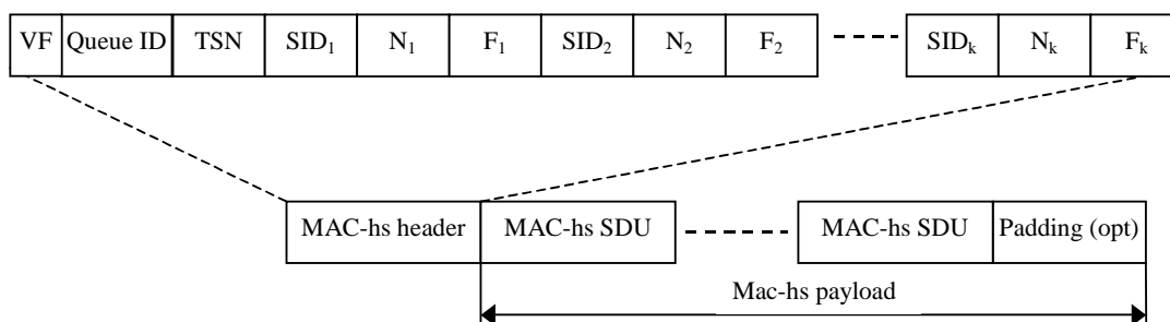
Figure 9.1.4.1: MAC-hs PDU
