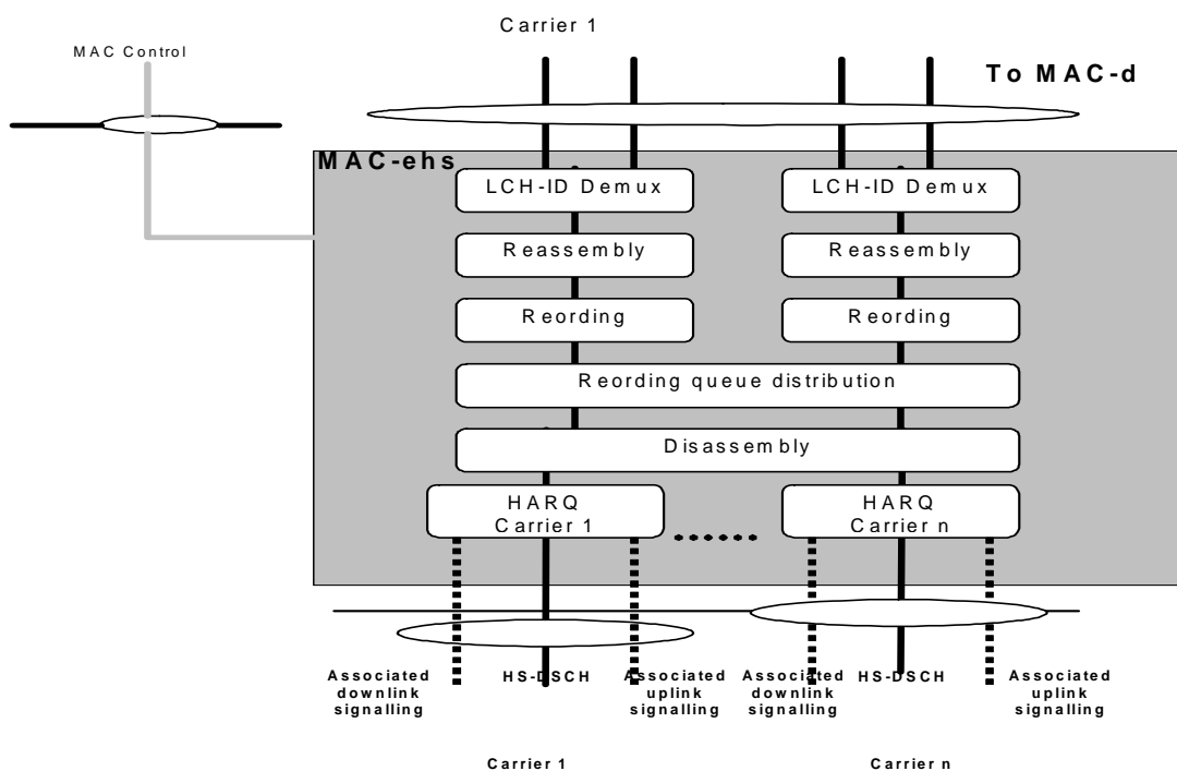
Figure 4.2.3.5-2: UE side MAC architecture/MAC-ehs details (1.28Mcps TDD multi-frequency HS-DSCH operation mode only)
