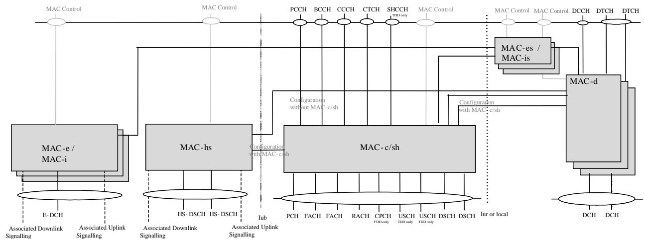
Figure 4.2.4.1: UTRAN side MAC architecture
