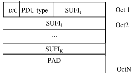
Figure 9.4: STATUS PDU
