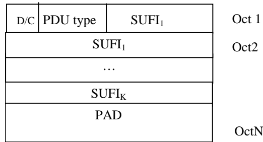
Figure 9.4: STATUS PDU
